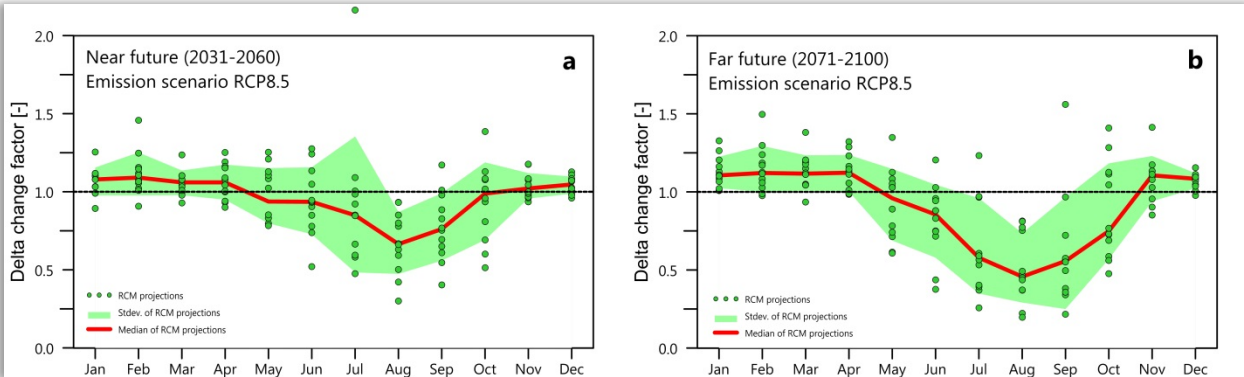
Fig 4. Projected changes in annual precipitation patterns for the GRRB. Values above one indicate a wetter future and below one a drier future.
