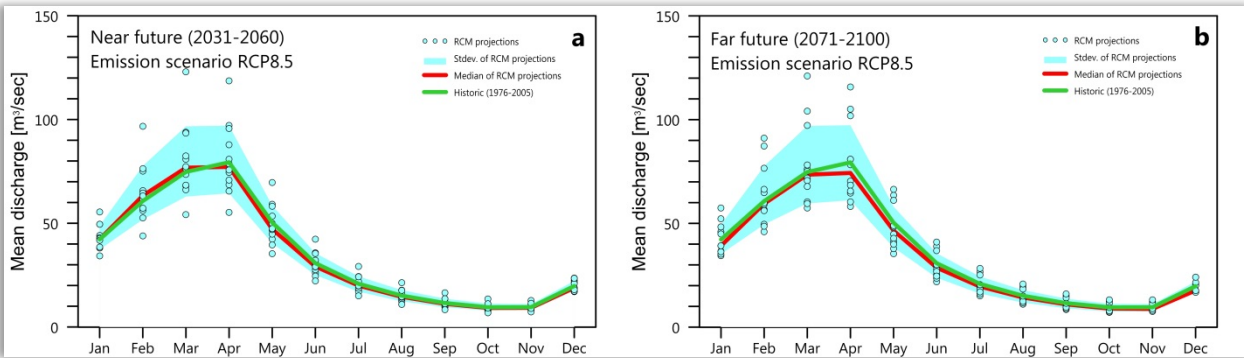
Fig 6. Projected changes in average monthly discharge at Iringa on the Little Ruaha River.
