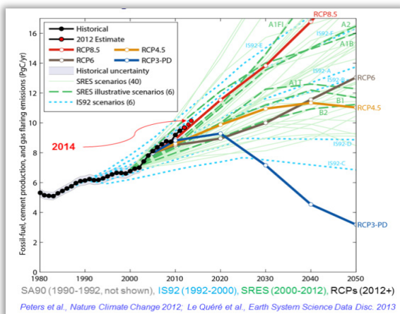
Fig 2. Greenhouse gas emission scenarios
