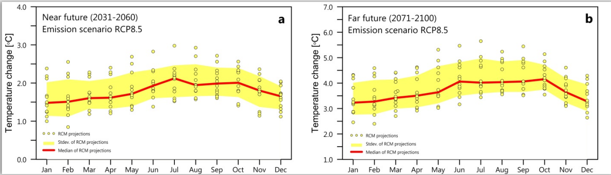
Fig 3. Projected changes in annual temperature patterns for the GRRB. Values reflect the increase in monthly mean temperature for the future.
