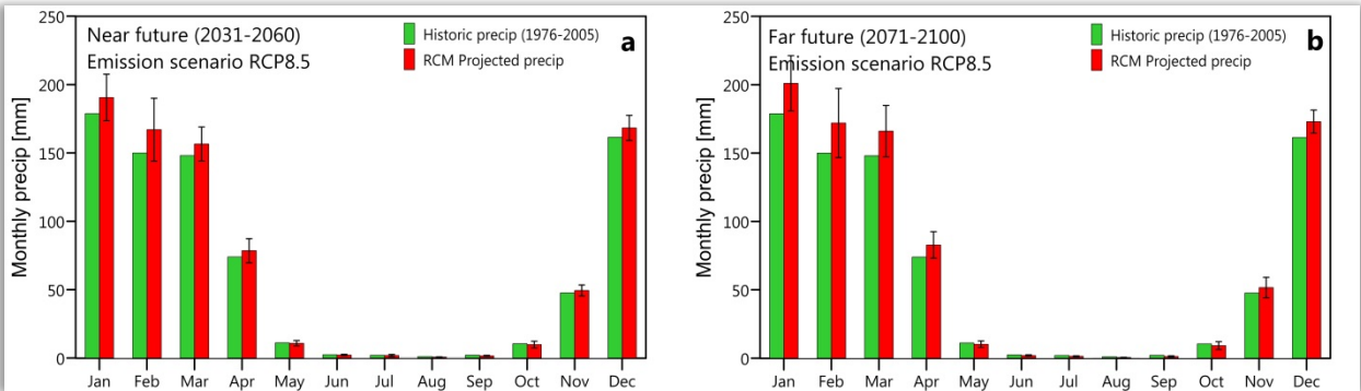
Fig 5. Projected changes in average monthly precipitation for the GRRB. Red bars represent the average of 12 RCM projections and the error bars the stdev. among the RCM's.
